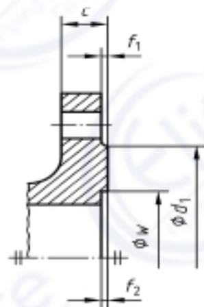
Type G: O-ring spigot
