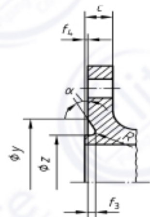
Type H: O-ring groove
