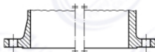
Type 21 Integral flange
