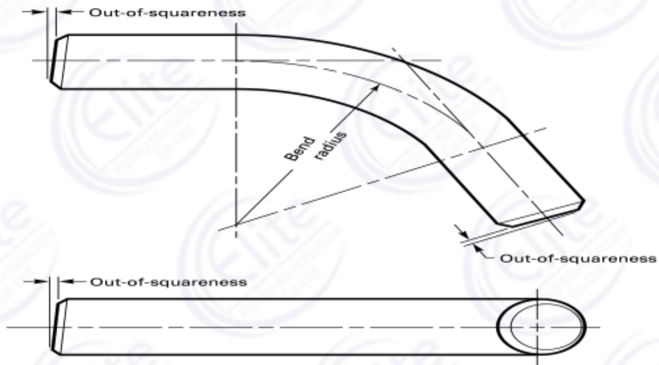
(b) Measurement of Out-of-Squareness
