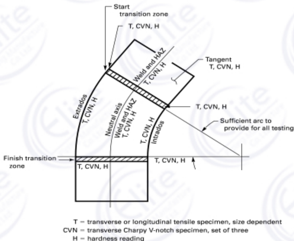
Figure 2 Test Specimen Locations and Orientations — Longitudinal Seam
