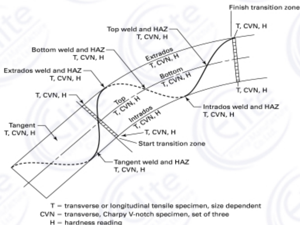
Figure 3 Test Specimen Locations and Orientations — Helical Seam
