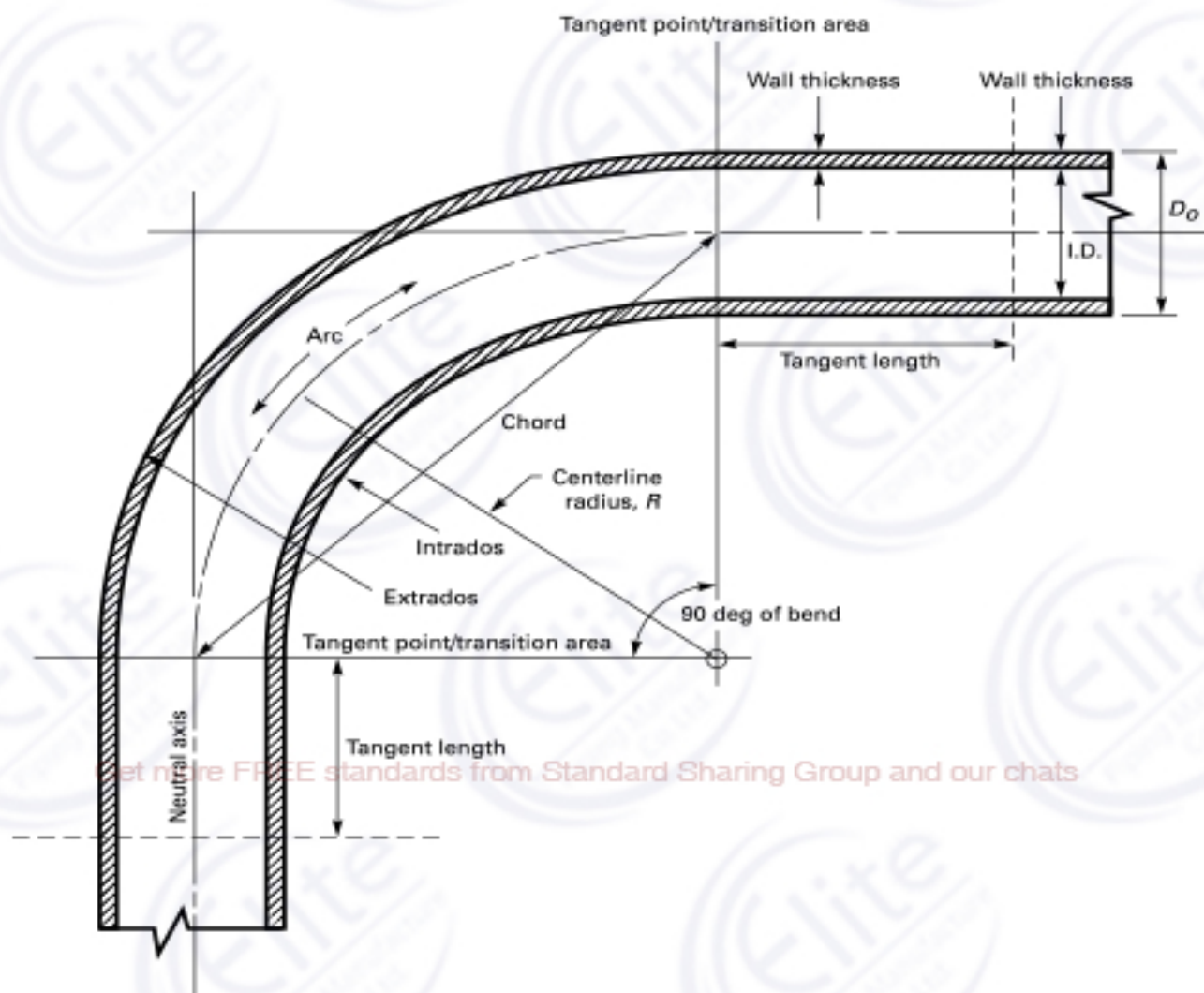
Figure 1 Bend Dimensional Terms
