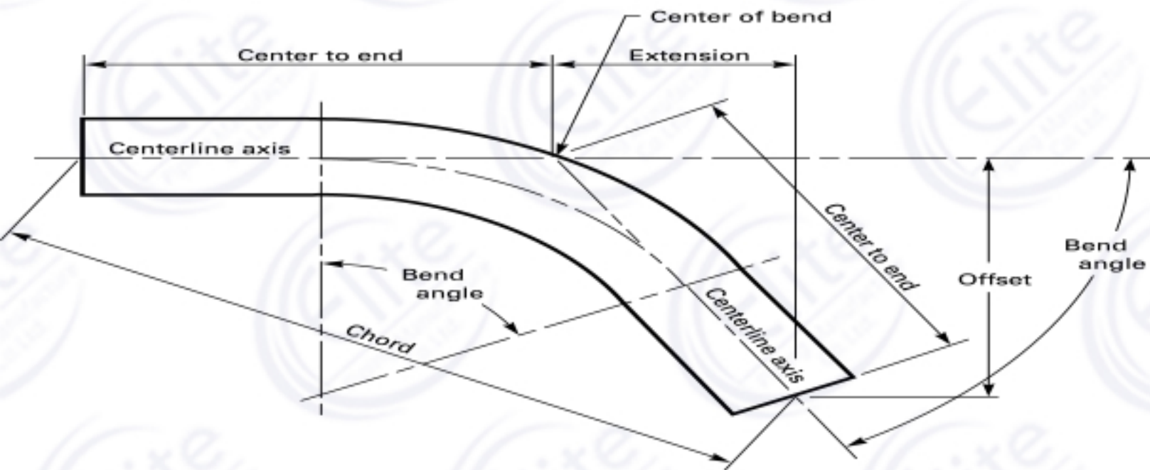
(a) Measurement of Bend Angle by Measurement and Calculation
